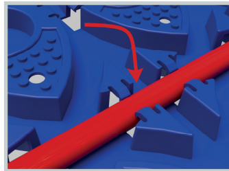
Multiple "PIPE RETENTION CLIPS" to secure the pipe in place.
